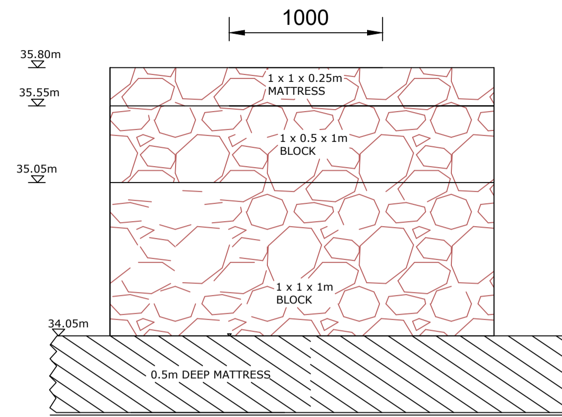
ELEVATION B-B SCALE - 1:25
